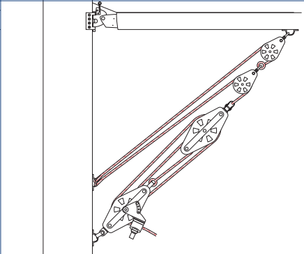
16:1 Cascaded kicker
