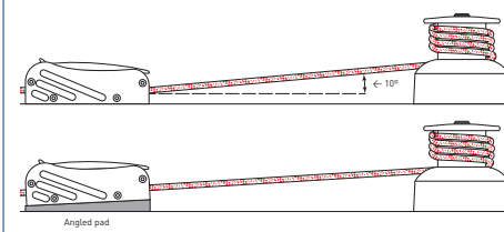
Clutch winch
