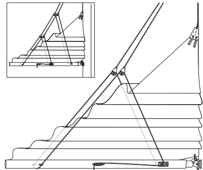
Lazy jacks
