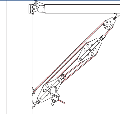
8:1 Cascaded kicker
